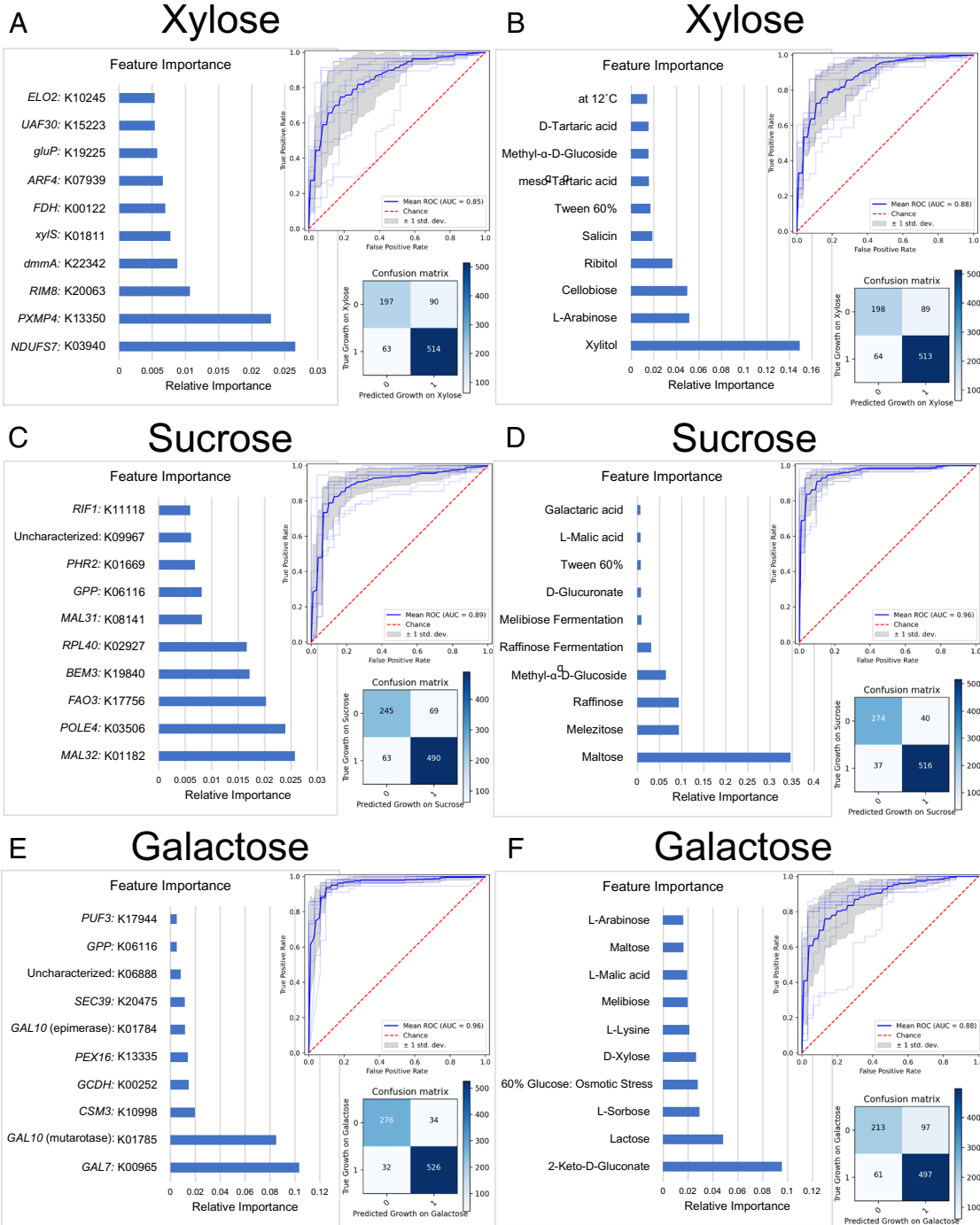
Fig. 3. Prediction accuracy of growth on different sugars was high when the random forest algorithm was trained on genomic data, and similarly high when the algorithm was trained on metabolic data. Panels (A) and (B): prediction of growth on xylose from genomic (A) or metabolic data (B). Panels (C) and (D): prediction of growth on sucrose from genomic (C) or metabolic (D) data. Panels (E) and (F): prediction of growth on galactose from genomic (E) or metabolic (F) data. Note that data on growth (and, where applicable, on fermentation) of the carbon source tested were removed prior to each analysis (e.g., prediction of growth on xylose from metabolic data was conducted using data for growth on all other substrates and conditions, but it excluded data for growth on xylose and xylose fermentation). Also note that KEGG Orthology misannotated GAL1 , likely leading GAL1 to not be in the top features, and that the epimerase and mutarotase domains encoded by GAL10 were annotated separately by this program. Accuracy is shown in the form of confusion matrices, which show strains predicted correctly to not grow on the sugar (true negatives, Top Left ), strains predicted to grow on the sugar that do not (false positives, Top Right ), strains correctly predicted to grow on the sugar (true positives, Bottom Right ), and strains predicted to not grow on the sugar that do (false negatives, Bottom Left ), as well as Receiver Operating Characteristic (ROC) curves, which show the true positive rate over false positive rate with changing classification thresholds. Feature importance graphs are also included to show the input features that are most useful for predicting growth on this sugar. XGBoost random forest was used to generate feature importance, and cross_val_predict() from sklearn.model_selection was used to generate confusion matrices. ROC curves were generated using the roc_curve function from sklearn.metrics . The prediction accuracies of growth on xylose, sucrose, and galactose from isolation environment data are shown in SI Appendix, Fig. S1 .
